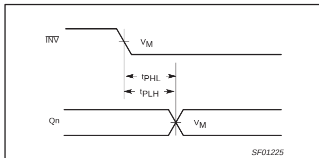
Waveform 3. Propagation Delay for \overline{\text{INV}} to Output
